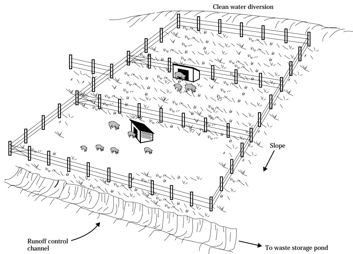
Figure 9-14 Runoff control
