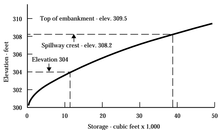
Figure 13-1 Stage-storage curve
